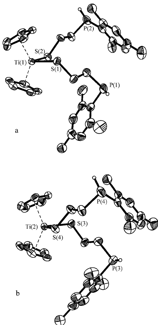
Figure 1. Molecular structure of [\text{Cp}_2\text{Ti}(\text{SCH}_2\text{CH}_2\text{PHMe}_2)_2] (5) showing the atom numbering scheme employed (ORTEP, 50% probability, SHELXTL PLUS; XP); [70] a) rac isomer; b) meso isomer; hydrogen atoms (other than P–H) are omitted for clarity
