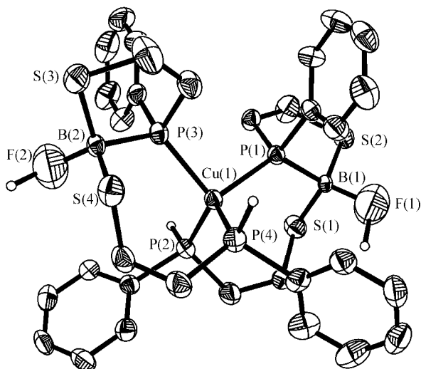
Figure 2. Molecular structure of (R_P, R_P, R_P, R_P, R_B, R_B)/(S_P, S_P, S_P, S_P, S_B, S_B)-[\text{Cu}\{P, P'-\text{PHPhCH}_2\text{CH}_2\text{SB}(\text{FH})\text{SCH}_2\text{CH}_2\text{PPh}(\text{B}-P)\}_2]\text{BF}_4 ( 7 ) showing the atom numbering scheme employed (ORTEP, 50% probability, SHELXTL PLUS; XP); [70] only the cation is shown; hydrogen atoms (other than P–H or F–H) are omitted for clarity
